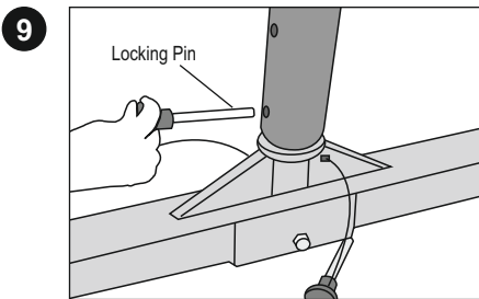
STEP 8- Lock the column leg on H-Base column using locking pin.
